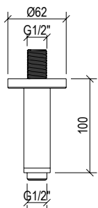
Braccio doccia a soffitto lungo 100 mm in acciaio inox 316L, con connessione G1/2". 100 mm long ceiling-mounted shower arm in 316L stainless steel, with G1/2" connection.
