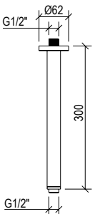
Braccio doccia a soffitto lungo 300 mm in acciaio inox 316L, con connessione G1/2". 300 mm long ceiling-mounted shower arm in 316L stainless steel, with G1/2" connection.
