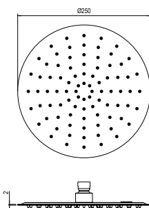
Soffione doccia tondo, diametro 250 mm, in acciaio inox 304L, con ugelli anticalcare e connessione con snodo a sfera G1/2". Round shower head, 250 mm diameter, in 304L stainless steel, with anti-limescale nozzles and G1/2" ball joint connection.
