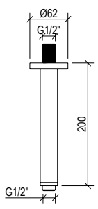
Braccio doccia a soffitto lungo 200 mm in acciaio inox 316L, con connessione G1/2". 200 mm long ceiling-mounted shower arm in 316L stainless steel, with G1/2" connection.
