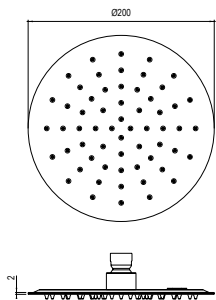
Soffione doccia tondo, diametro 200 mm, in acciaio inox 304L, con ugelli anticalcare e connessione con snodo a sfera G1/2". Round shower head, 200 mm diameter, in 304L stainless steel, with anti-limescale nozzles and G1/2" ball joint connection.
